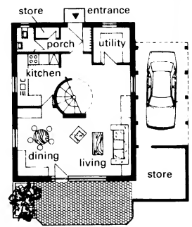
8 Ground floor
